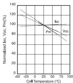
Normalized Isc, Voc, Pm vs. Cell Temperature Characteristics
